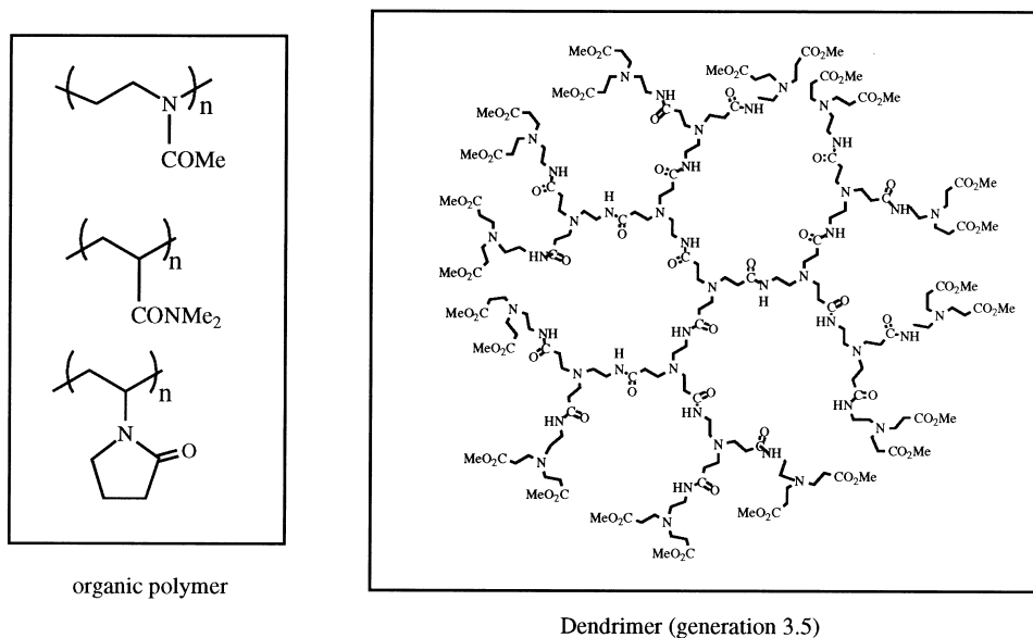
Fig. 1. Template macromolecules.
